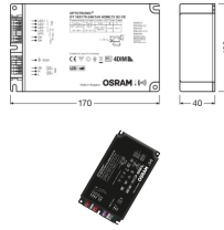
Technische Daten Osram Optotronic LED Driver OT 165/170-240/1A0 4DIMLT2 G2 CE
